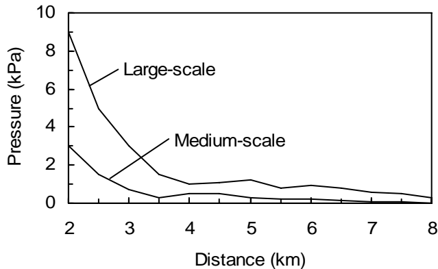
Figure 10. Dynamic pressures produced by pyroclastic flows along the southern slope of Vesuvius at 10 m above the ground. The input parameters for large- and medium-scale eruptions are those as described in Dobran et al. (1994). A large-scale eruption discharges about 10^8 and medium-scale 10^7 kg/s of material.
