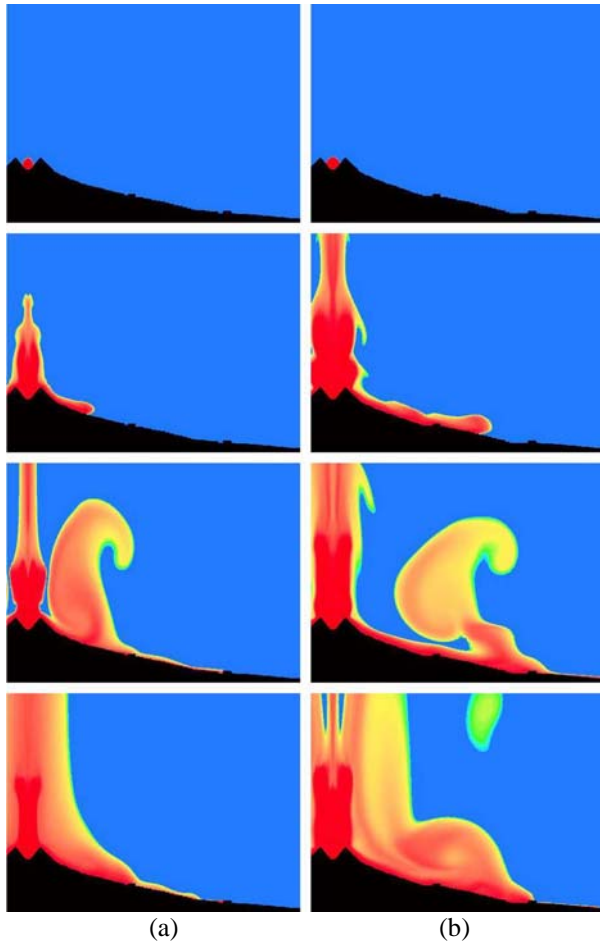
Figure 8. (a) Pyroclastic flow from a subplinian eruption can be stopped by a 30-m-high obstacle at 5 km from the vent. Frames shown correspond to 0, 30, 300, and 900 s after the eruption. (b) Pyroclastic flow from a plinian eruption can also be slowed down considerably by this obstacle. Frames shown correspond to 0, 180, 300, and 400 s after the eruption.
