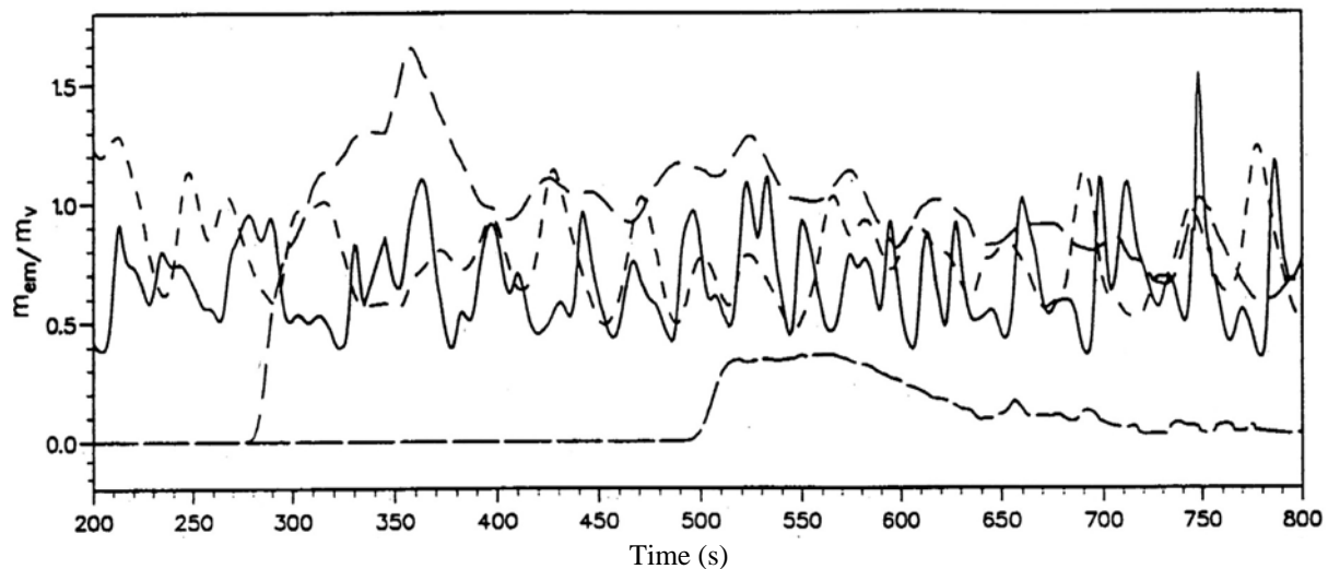
Figure 11. Timewise distributions of pyroclastic mass flow rates normalized by the steady-state discharge mass flow rate of a large-scale eruption of Vesuvius. R = 3 (solid line), 6 (short dashed line), 10 (medium dashed line), and 15 km (long dashed line) from the vent. Velocities, densities, and other parameters exhibit similar fluctuations.
