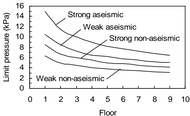
Figure 9. Horizontal limit pressures of strong and weak buildings constructed according to aseismic and non-aseismic building codes. Adapted from Petrazzuoli & Zuccaro (2004).
