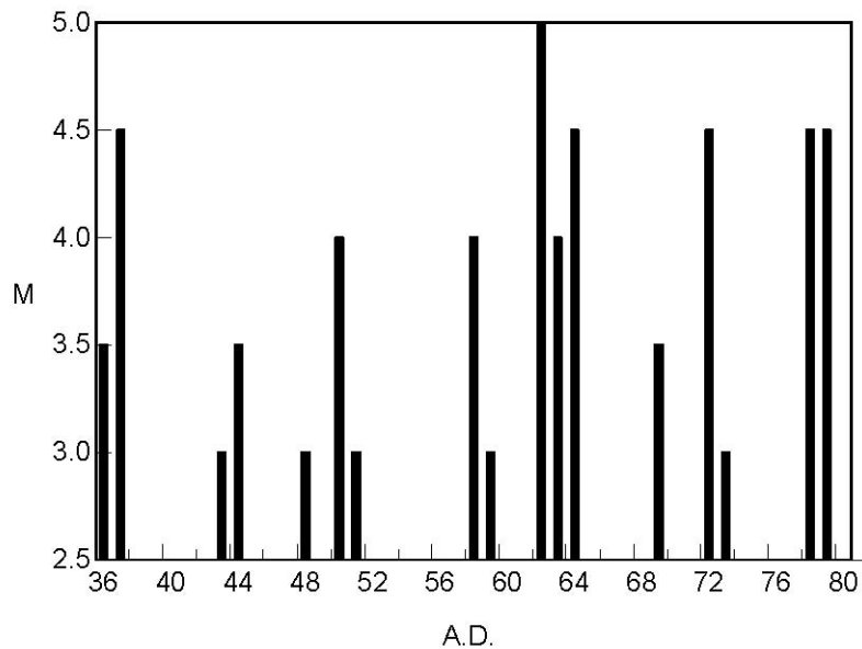
Figure 3. Estimated magnitudes of earthquakes preceding the eruption of 79 A.D. Earthquakes from historical sources include those that are dated (37, 62, 64, 79 A.D.) and those that are not dated. Earthquakes from archaeological sources (62, 72, 78, 79 A.D.) are responsible for damages. Adapted from Marturano (2006).
