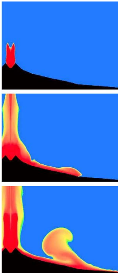
Figure 7. A large-scale eruption of Vesuvius discharges about 10^8 kg/s of material and produces collapses of the volcanic column. The collapsed column produces pyroclastic flows which in about 5 minutes reach the Tyrrhenian Sea. Frames shown correspond to 20, 120, and 300 s after the eruption. The red color denotes high concentrations or temperatures of pyroclasts.
