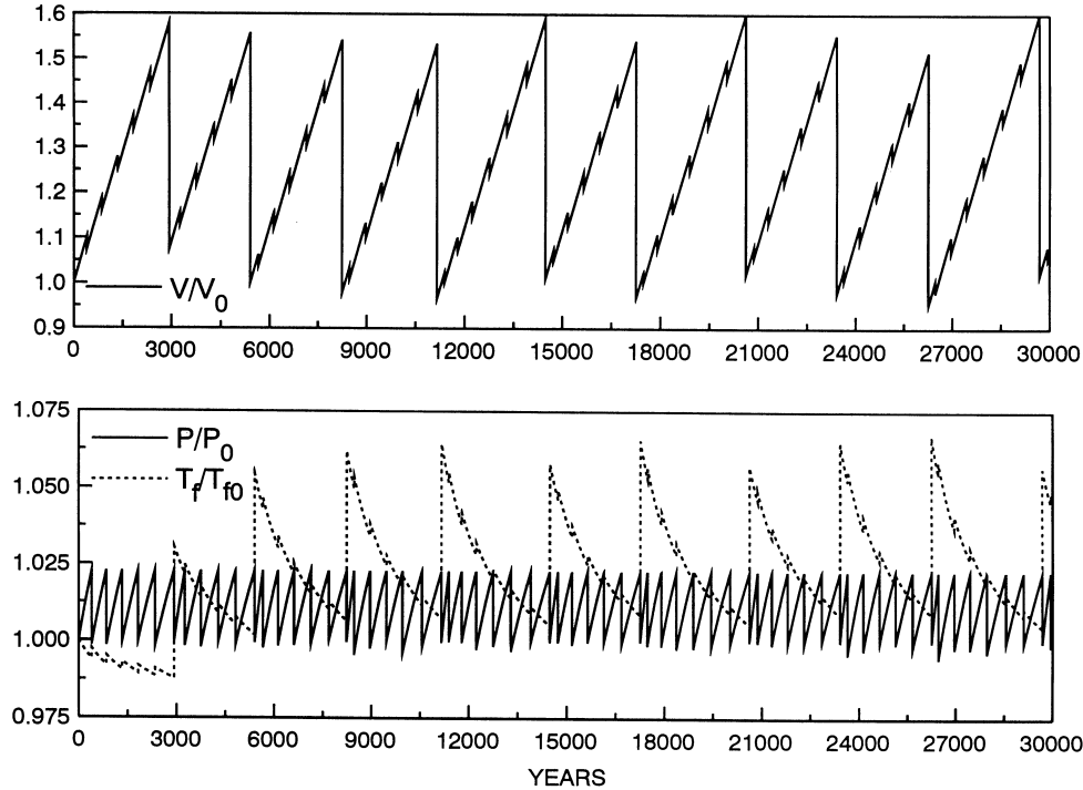
Figure 6. The simulator’s magma chamber dynamics model (Dobran 2001) predicts a subplinian or plinian eruption of Vesuvius during this century. Plinian eruptions occur in cycles of several thousand years. Several subplinian eruptions with increasing periods occur between any two plinian eruptions. The results are expressed in terms of the normalized volume, pressure, and temperature of magma in the chamber as a function of time. After several thousand years the initial conditions for simulations do not determine the long-term system behavior.
