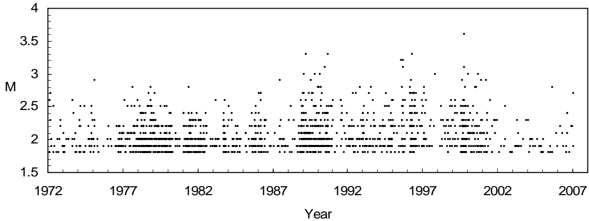
Figure 5. Distribution of recent earthquakes at Vesuvius with M \geq 1.8 . Adapted from De Natale et al. (2004a) using earthquake catalog data of Osservatorio Vesuviano.
